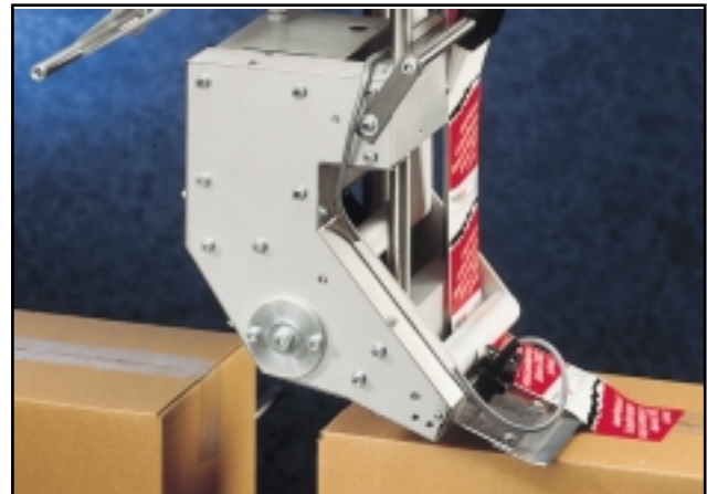
Fast speed labelling head for speed up to 100 m/min
